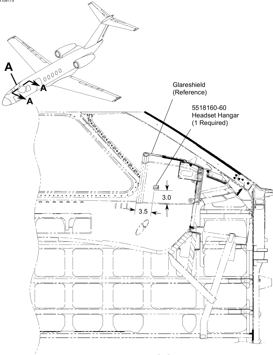
VIEW A-A Looking Outboard Left Side Shown, Right Side Oppsite
