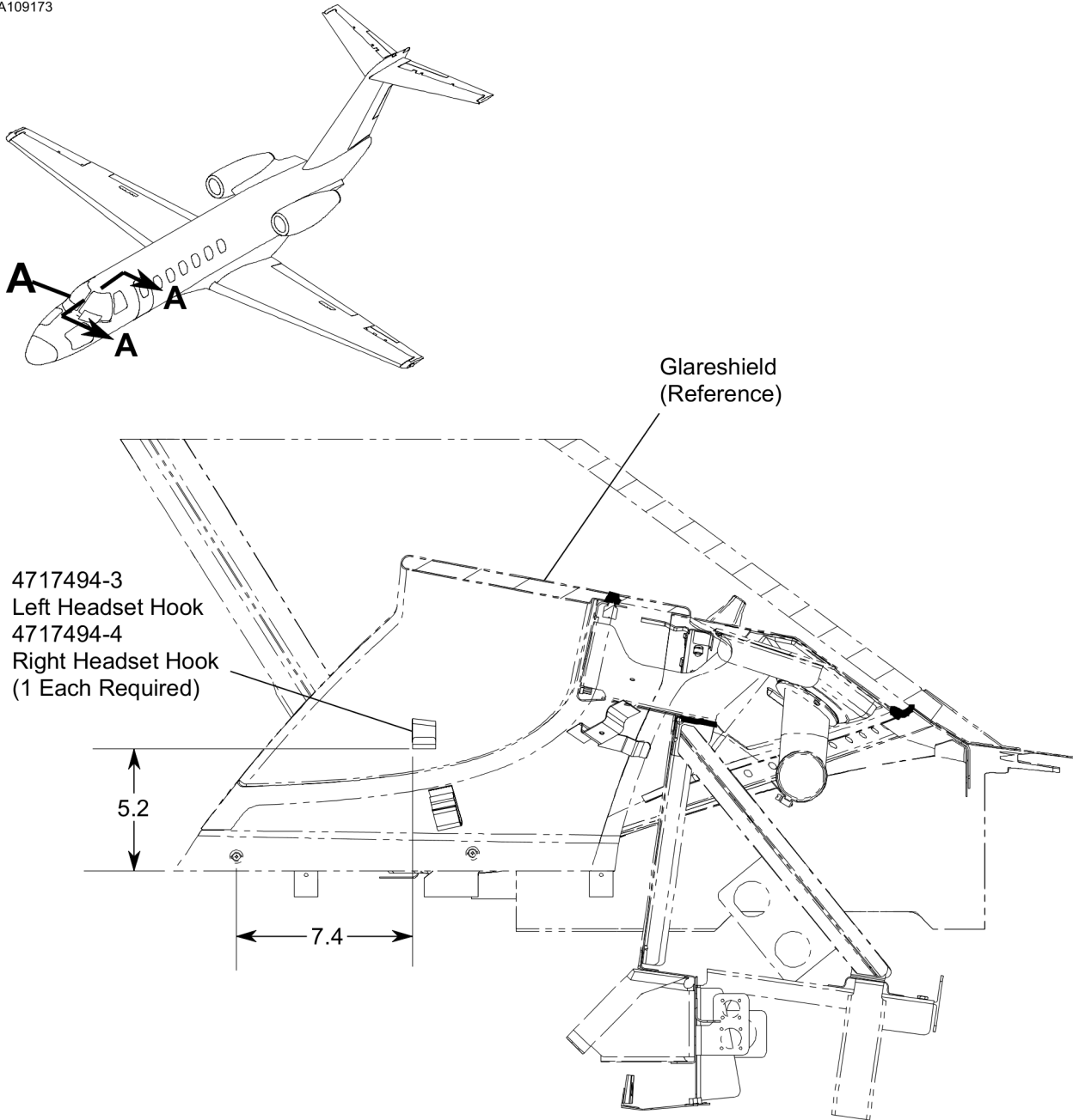
VIEW A-A Looking Outboard Left Side Shown, Right Side Opposite
